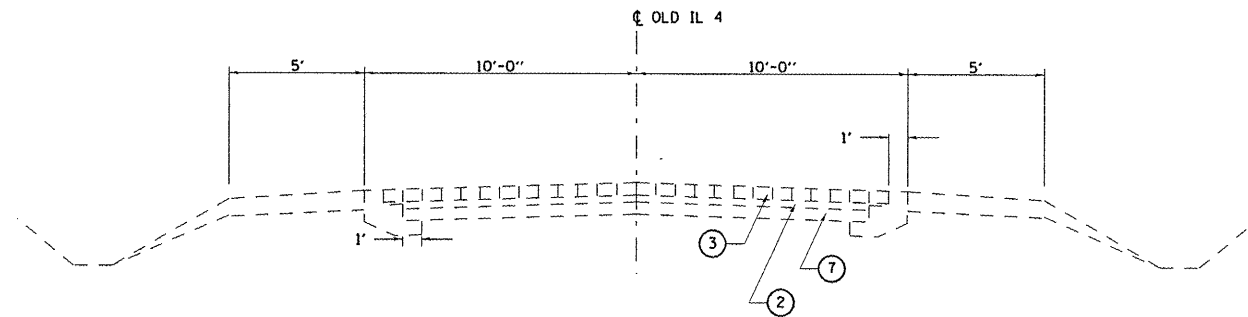
EXISTING TYPICAL CROSS SECTION ① OLD IL 4
