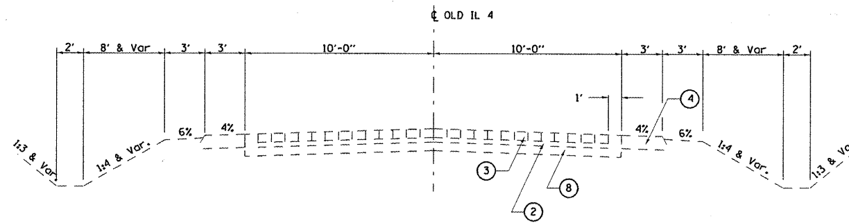
EXISTING TYPICAL CROSS SECTION ② OLD IL 4
