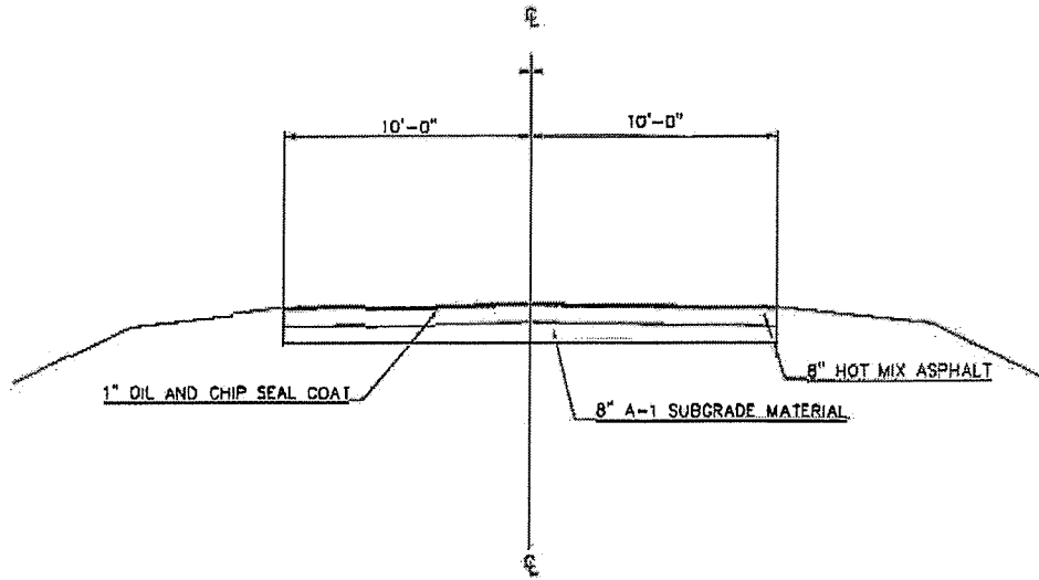
EXISTING TYPICAL CROSS SECTION
