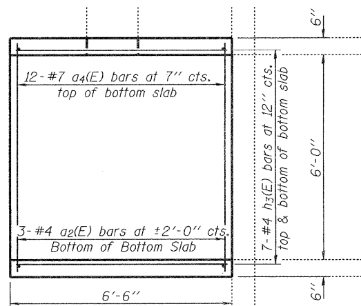
PLAN BOTTOM SLAB
