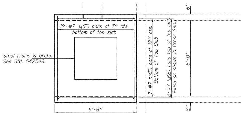
PLAN TOP SLAB Cut a 4 (E) & h 2 (E) bars as required to clear grate.
