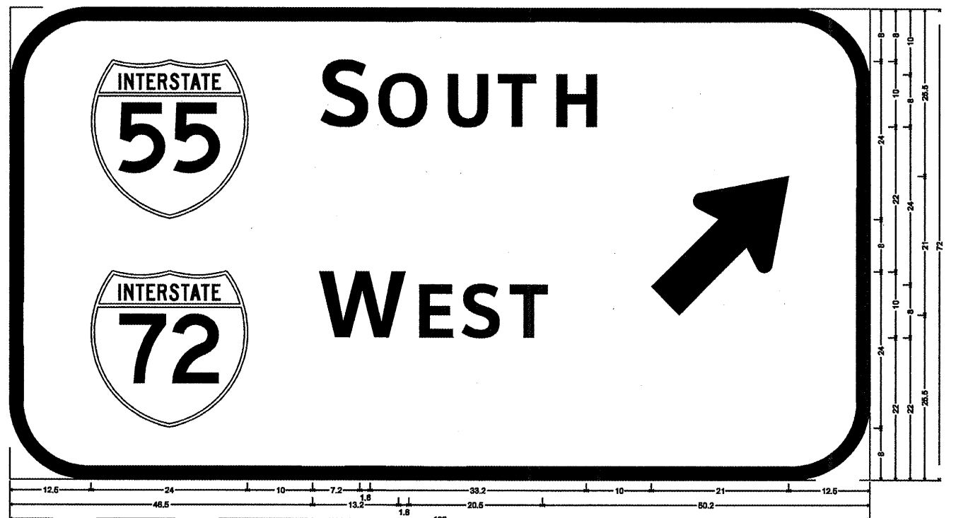
12.0" Radius, 2.0" Border, White on Green; Interstate 55 10.7" D; [S SOUTH] Clearview Hwy-S-W; Interstate 72 10.7" D; [W WEST] Clearview Hwy-S-W; Standard Arrow Custom 28.8" X 18.1" 45°;
