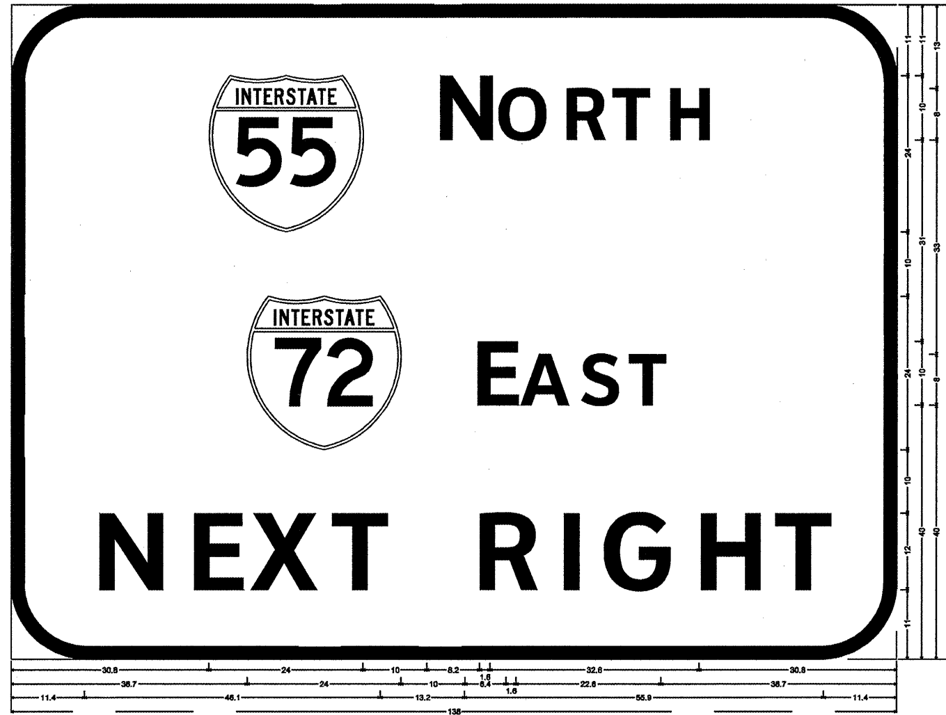
12.0" Radius, 2.0" Border, White on Green; Interstate 55 10.7" D; [N ORTH] Clearview Hwy-S-W; Interstate 72 10.7" D; [E EAST] Clearview Hwy-S-W; [NEXT RIGHT] Clearview Hwy-S-W;
