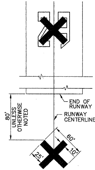
CLOSED RUNWAY MARKER DETAIL N.T.S.
