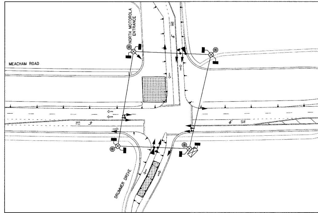
MAINTENANCE OF TRAFFIC STAGE III-C
