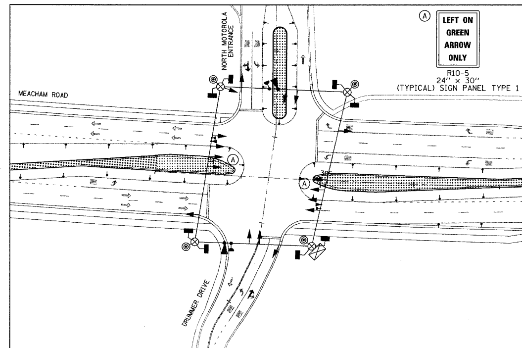
MAINTENANCE OF TRAFFIC STAGE IV
