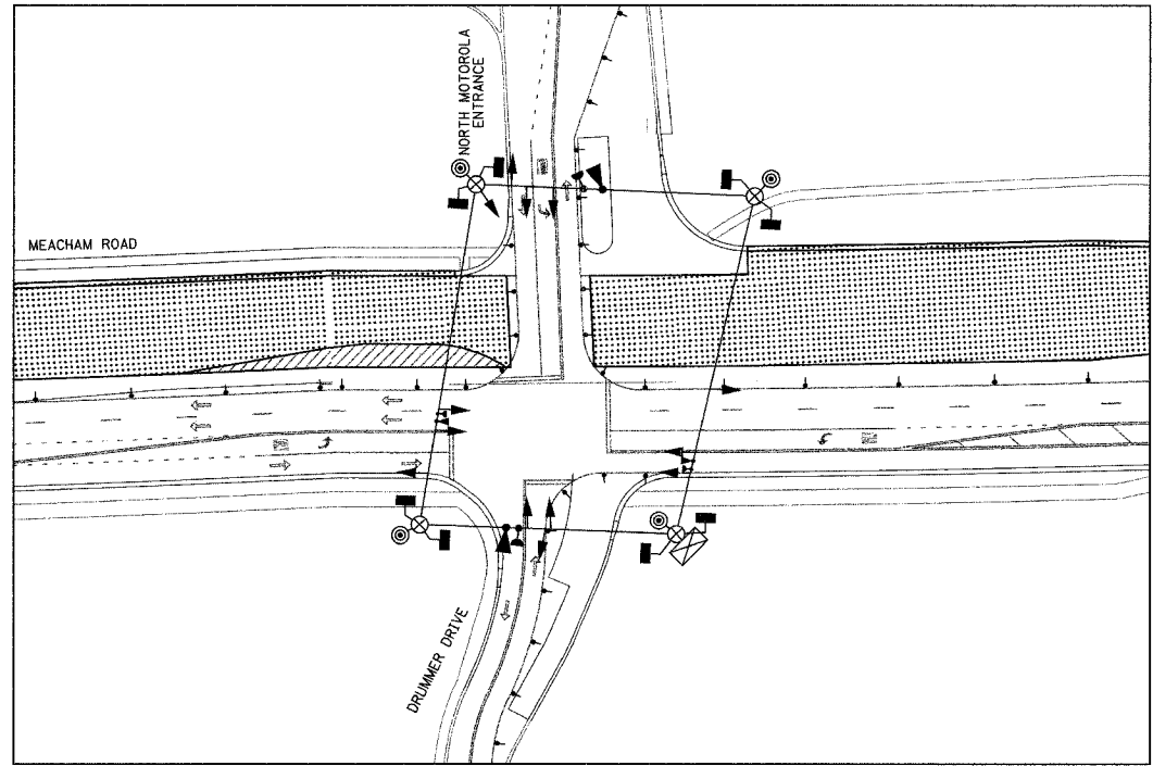
MAINTENANCE OF TRAFFIC STAGE III-B
