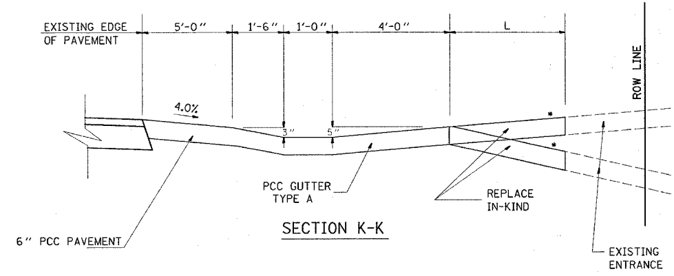
CE & SR DETAIL K COMMERCIAL & SIDE ROAD ENTRANCE ADJACENT TO BITUMINOUS SHOULDER AND PCC GUTTER TYPE A
