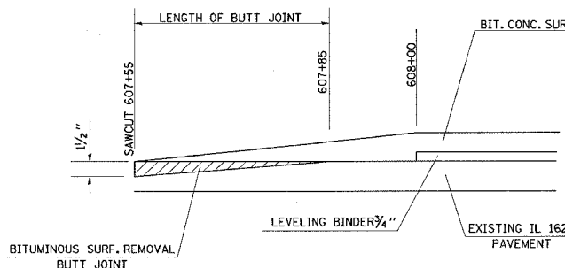
BUTT JOINT DETAIL STA. 608+00
