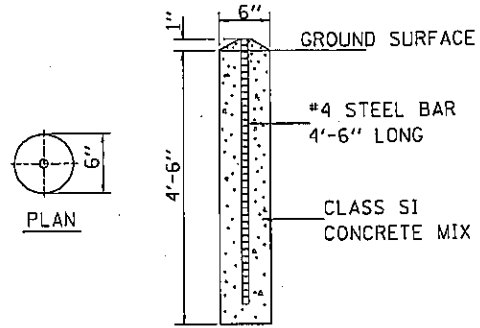
CONCRETE REFERENCE MARKER
