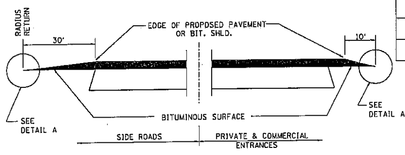
SECTION A-A DETAILS AT ENTRANCES & SIDE ROADS
