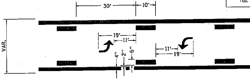
TYPICAL APPLICATION @ BI-DIRECTIONAL TURN LANE
