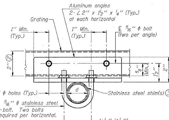
SECTION T-T
