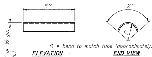
SHIM DETAIL
