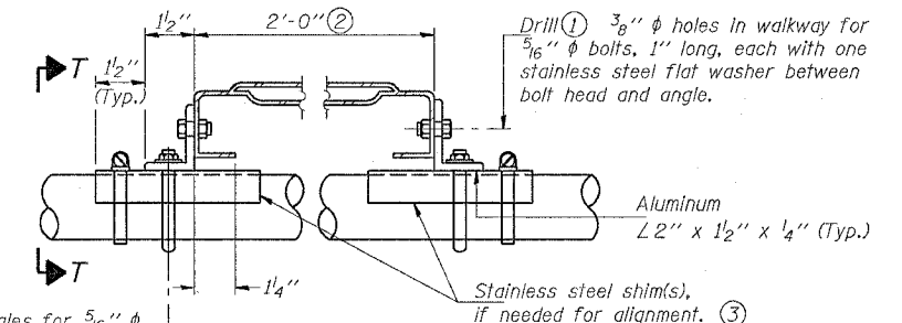
DETAIL T
