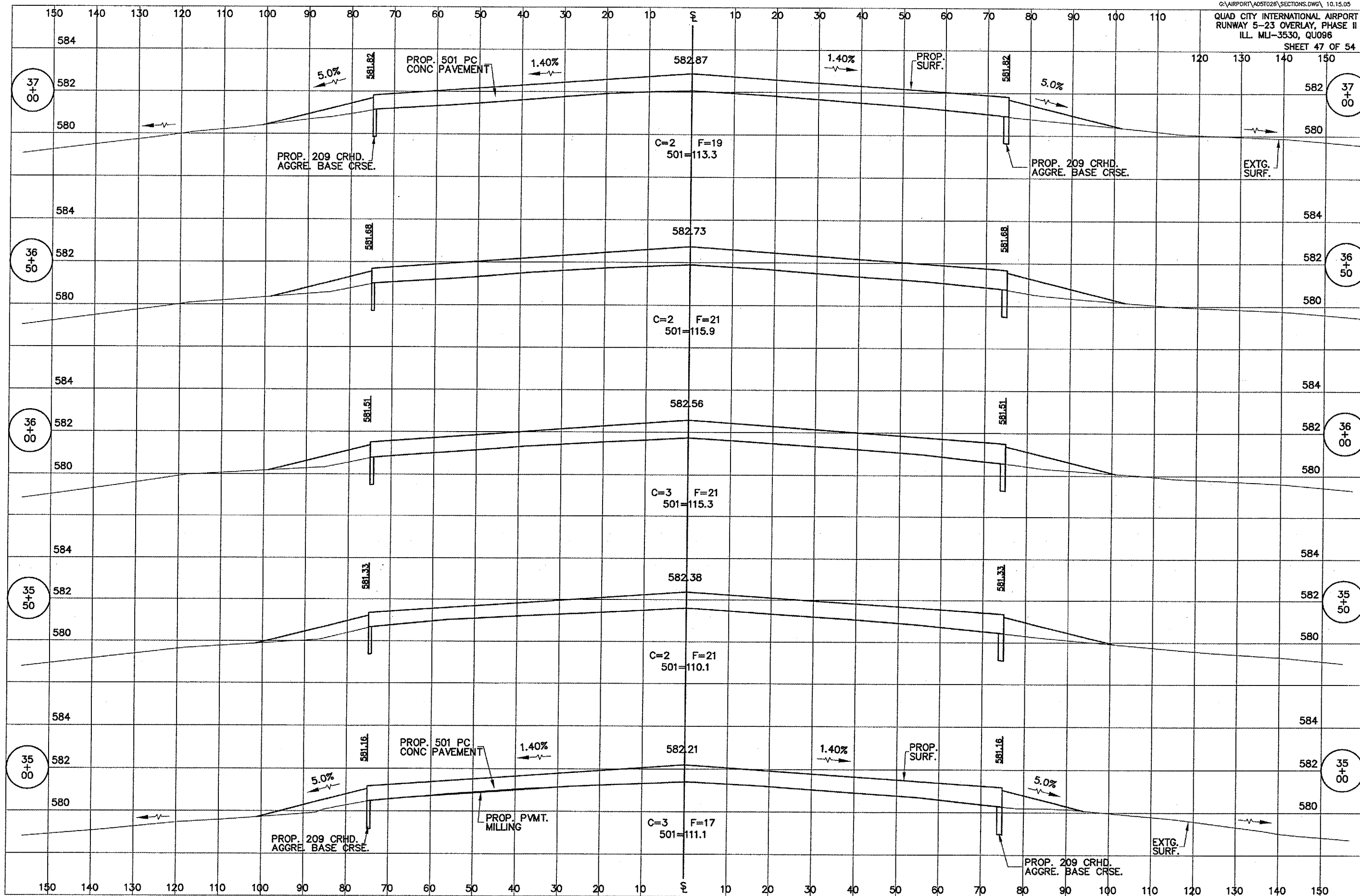
RUNWAY 5-23 OVERLAY CROSS SECTIONS, STA 35+00 TO STA 37+00
