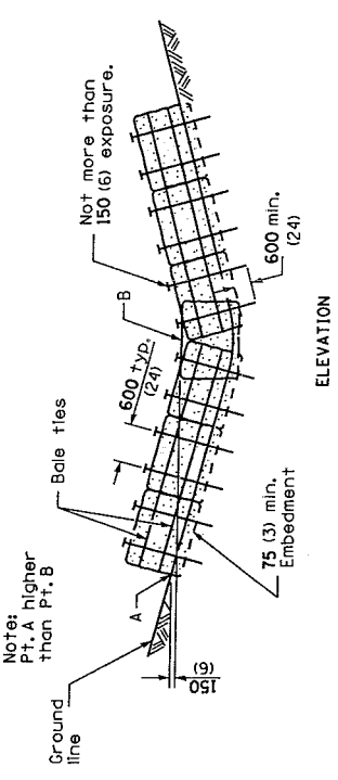
ROLLED EXCELSIOR OR STRAW BALES FOR DITCH CHECK
