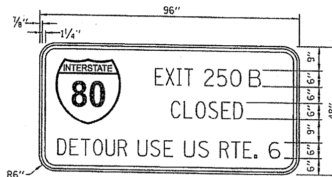
SIGN DETAIL NO. 4 SIGN PANEL - TYPE 3
