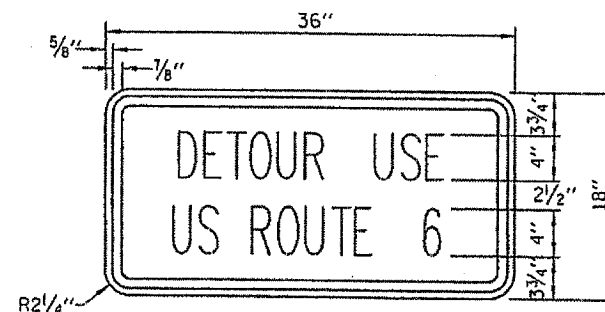
SIGN DETAIL NO. 1 SIGN PANEL - TYPE 1
