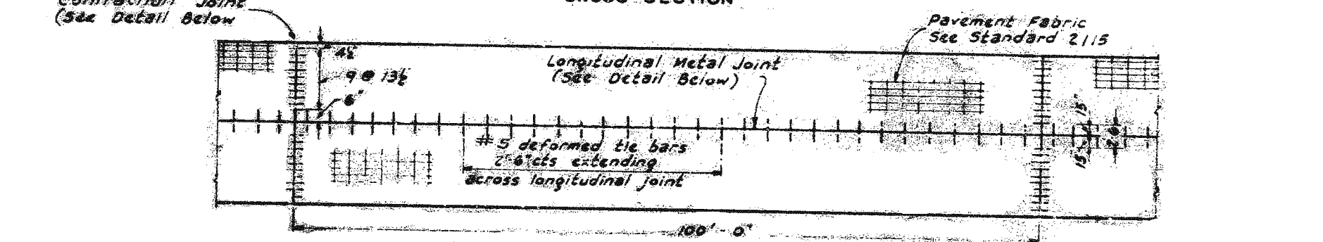
PLAN FOR P.C. CONCRETE PAVEMENT
