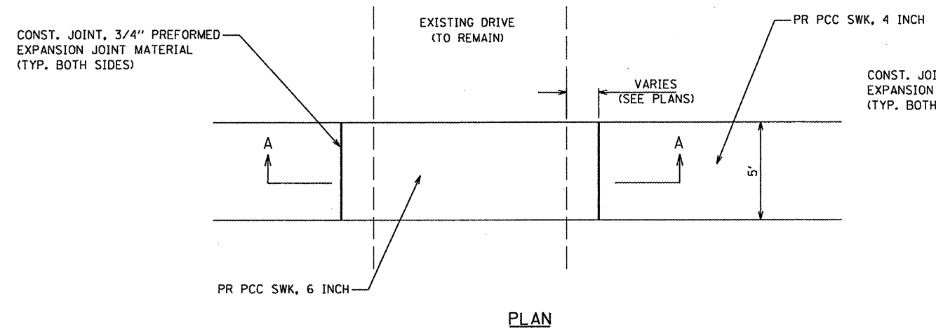
PROPOSED PCC SIDEWALK TRANSITION DETAIL ACROSS DRIVES NOT TO SCALE
