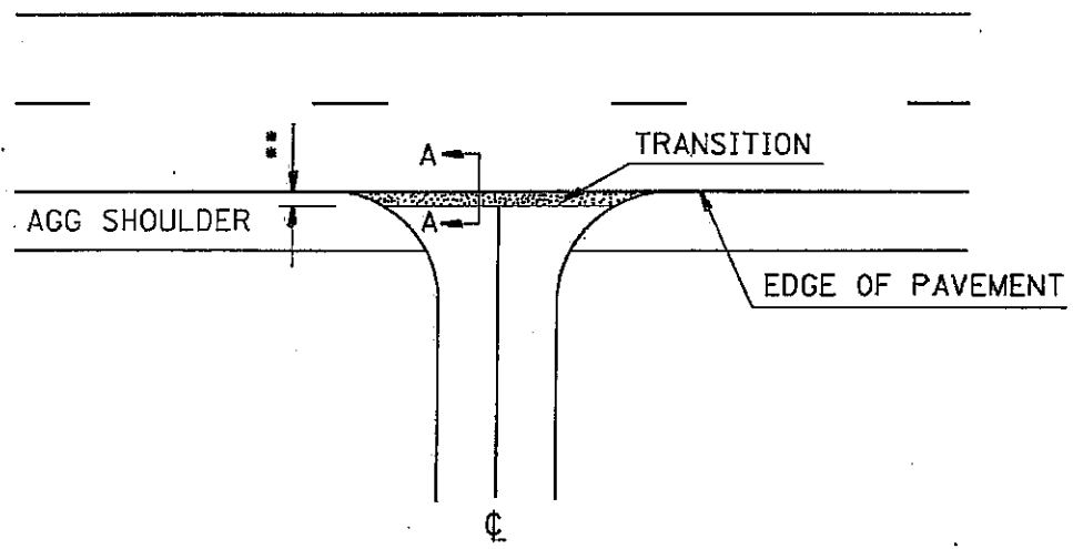
SIDEROAD DETAIL (EXCEPT AT N. FIRST ST.)
