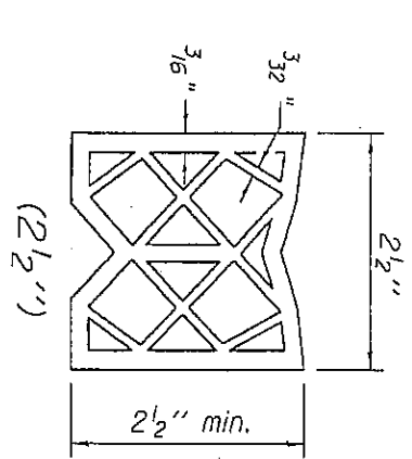
PREFORMED JOINT SEAL
