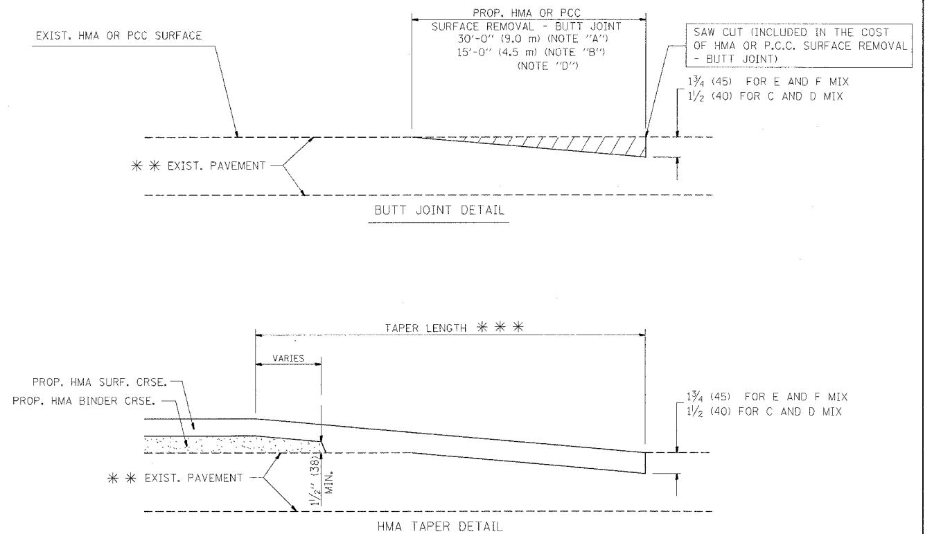
TYPICAL BUTT JOINT AND HMA TAPER FOR RESURFACING ONLY
