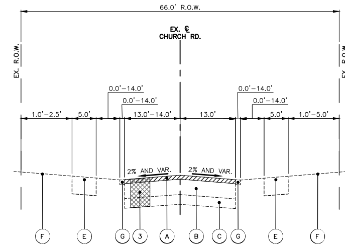
EXISTING TYPICAL SECTION - CHURCH RD. STA: 16+53 - STA: 27+50
