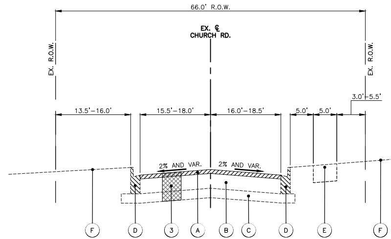
EXISTING TYPICAL SECTION - CHURCH RD. STA: 3+00 - STA: 16+53
