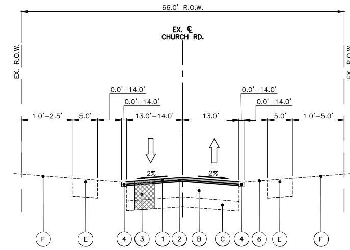
PROPOSED TYPICAL SECTION - CHURCH RD. STA: 16+53 - STA: 27+50
