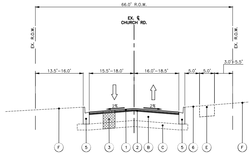
PROPOSED TYPICAL SECTION - CHURCH RD. STA: 3+00 - STA: 16+53
