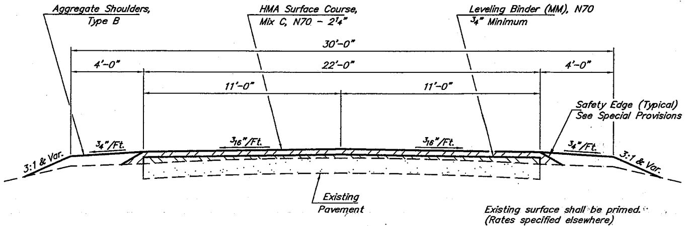
TYPICAL SECTION
