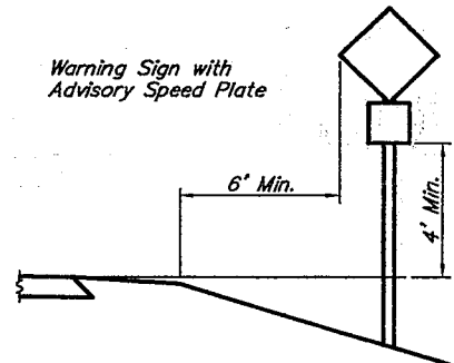
Warning Sign with Advisory Speed Plate
