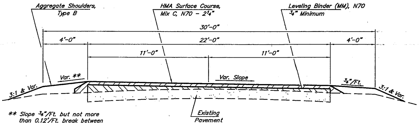
TYPICAL SECTION THRU CURVES
