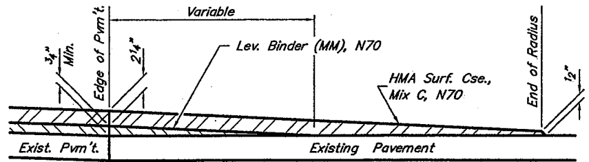
SECTION A-A SIDE ROAD (Est. No. = 2)
