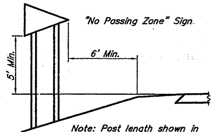
"No Passing Zone" Sign.
