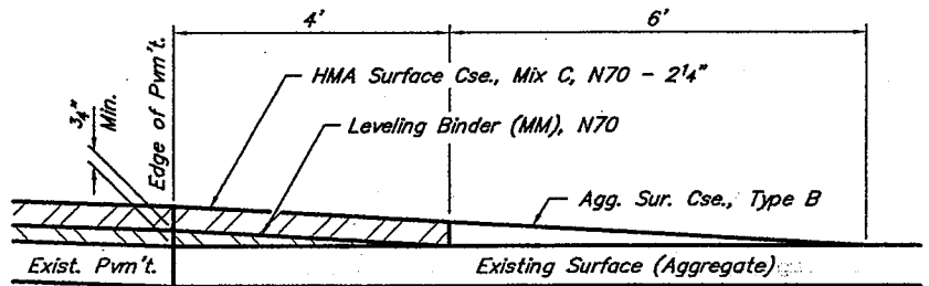
SECTION A-A PRIVATE ENTRANCE - AGGREGATE (Est. No. = 38)
