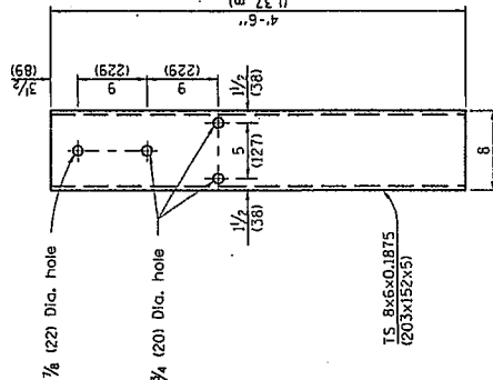
STEEL TUBE (2 ea.)
