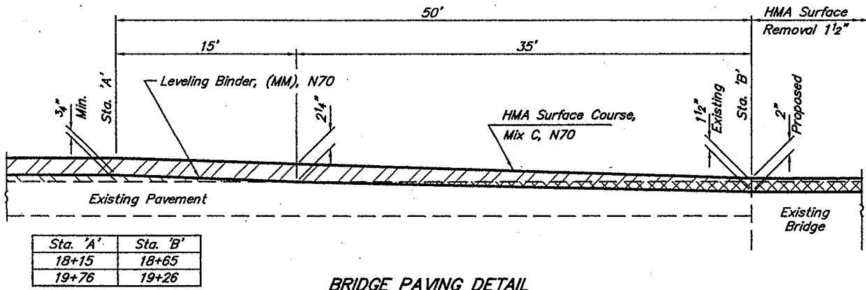
BRIDGE PAVING DETAIL
