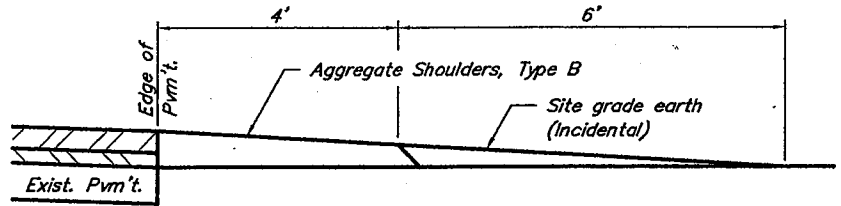
SECTION A-A FIELD ENTRANCE (Est. No. = 9)
