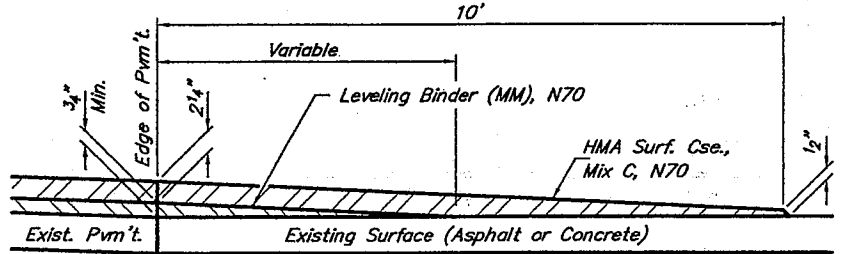
SECTION A-A PRIVATE ENTRANCE - ASPHALT (Est. No. = 7)
