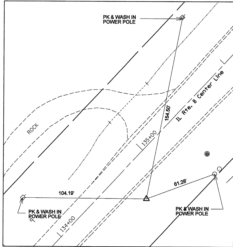
CONTROL POINT # 0304 STA 134+72.37, 30.41 RT
