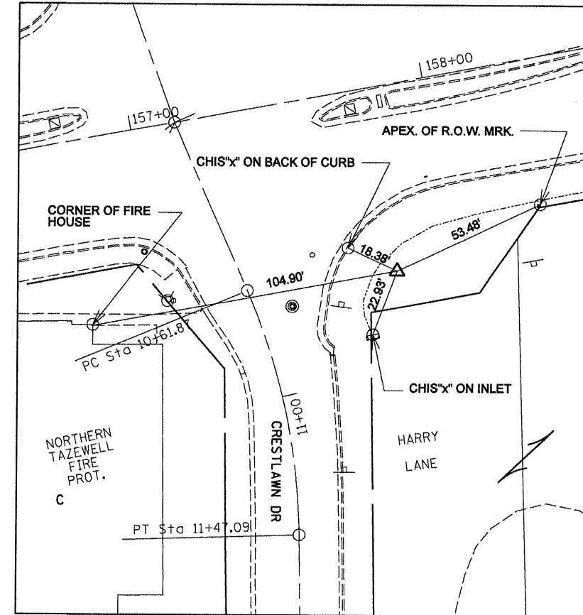
CONTROL POINT # 0310 STA 157+80.10, 62.92 RT
