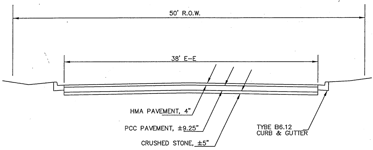
TYPICAL EXISTING SECTION STATION 0+00 TO 33+23
