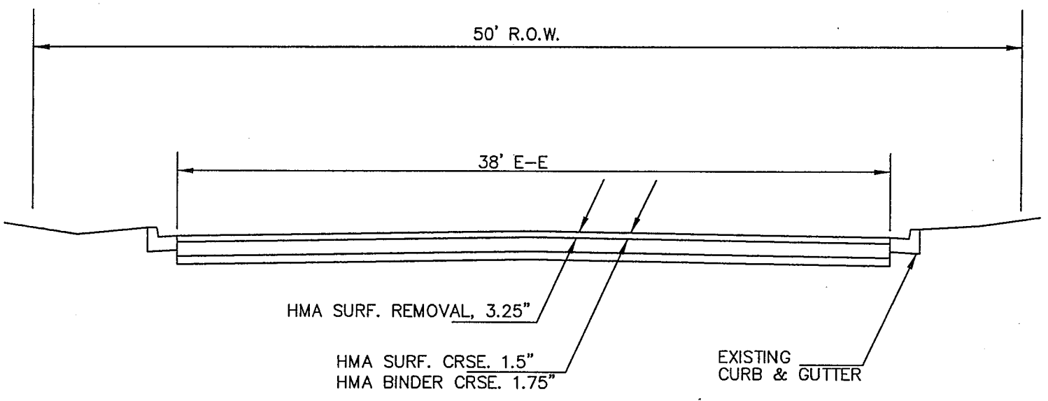
TYPICAL PROPOSED SECTION STATION 0+00 TO 33+23
