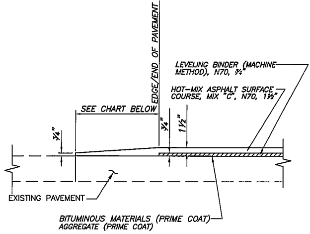
FEATHEREDGE DETAIL
