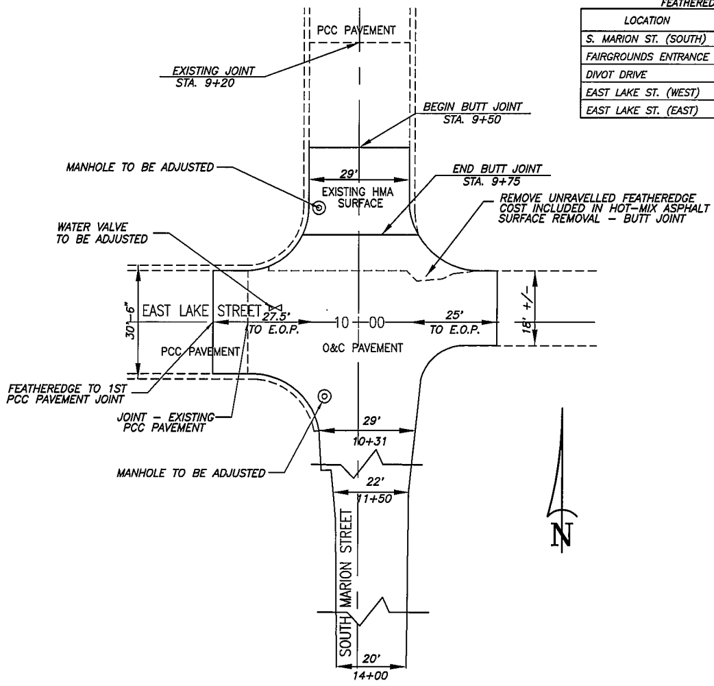
INTERSECTION DETAIL
