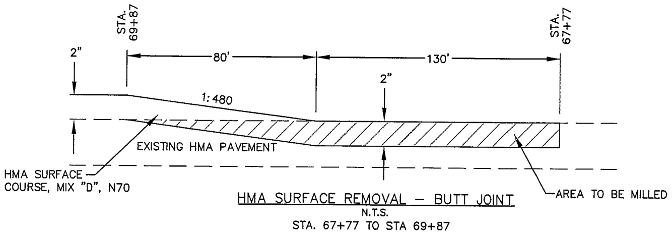
SIDE ROAD HMA SURFACING DETAIL N.T.S.
