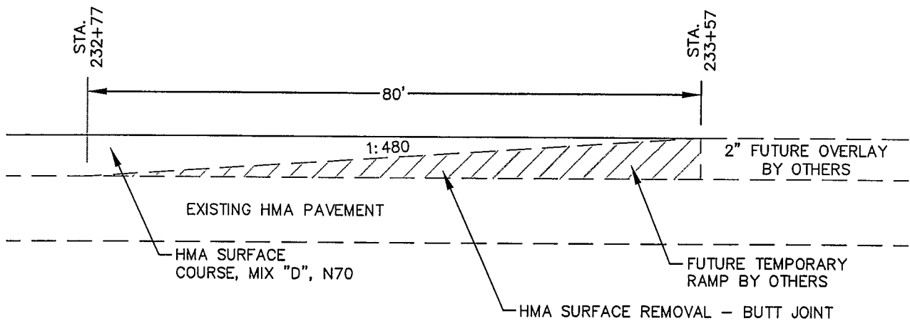
HMA SURFACE REMOVAL - BUTT JOINT N.T.S.
