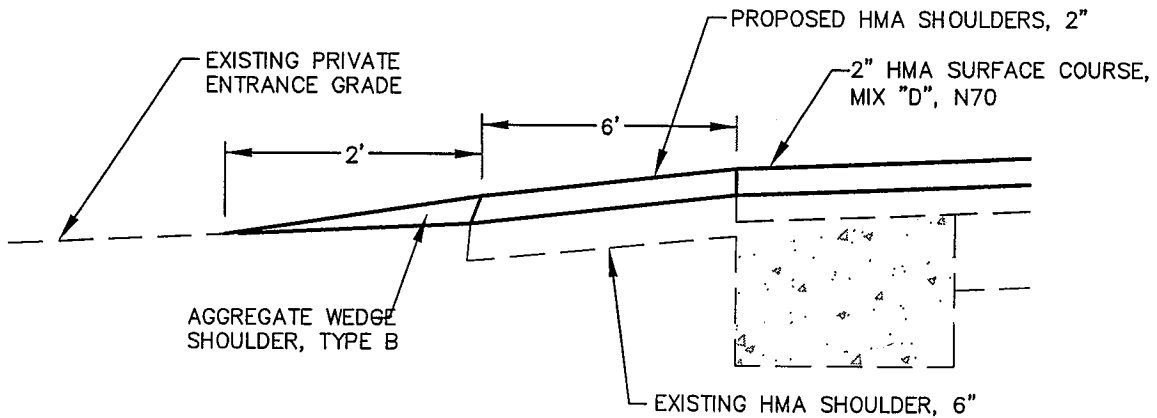
AGGREGATE PRIVATE ENTRANCE DETAIL -ELEVATION N.T.S.
