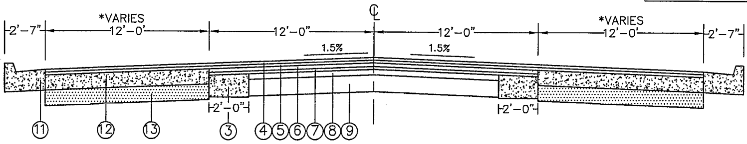
EXISTING TYPICAL SECTION STATION 0+24 TO 8+42.3 *BEGIN TAPER TO 2 LANES STATION 5+95
