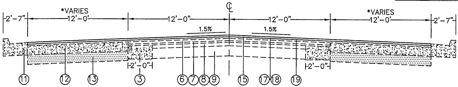
PROPOSED TYPICAL SECTION STATION 0+24 TO 8+42.3 *BEGIN TAPER TO 2 LANES STATION 5+95
