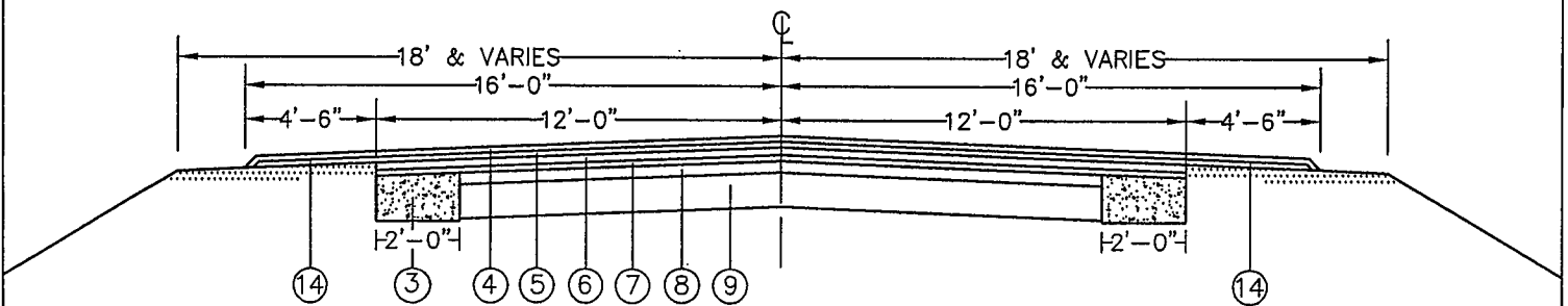
EXISTING TYPICAL SECTION STATION 42+00 TO 74+60
