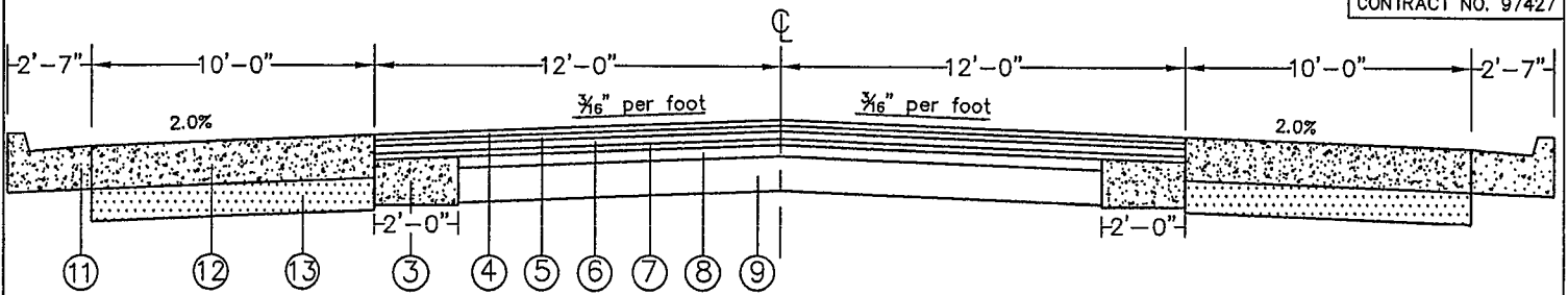
EXISTING TYPICAL SECTION LT. STATION 32+90 TO 42+00 RT. STATION 32+90 TO 37+15
