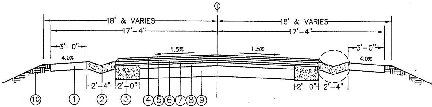
EXISTING TYPICAL SECTION STATION 8+42.3 TO 32+90 STATION 37+15 RT. TO 42+00 RT.
