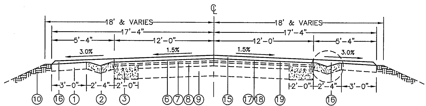
PROPOSED TYPICAL SECTION STATION 8+42.3 TO 32+90 STATION 37+15 RT. TO 42+00 RT.
