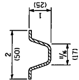
SECTION E-E 1.12 lbs./ft. Steel - (1.67 kg/m)
