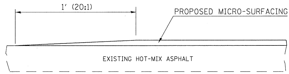
TAPER DETAIL FOR BEGINNING AND END OF PROJECT
