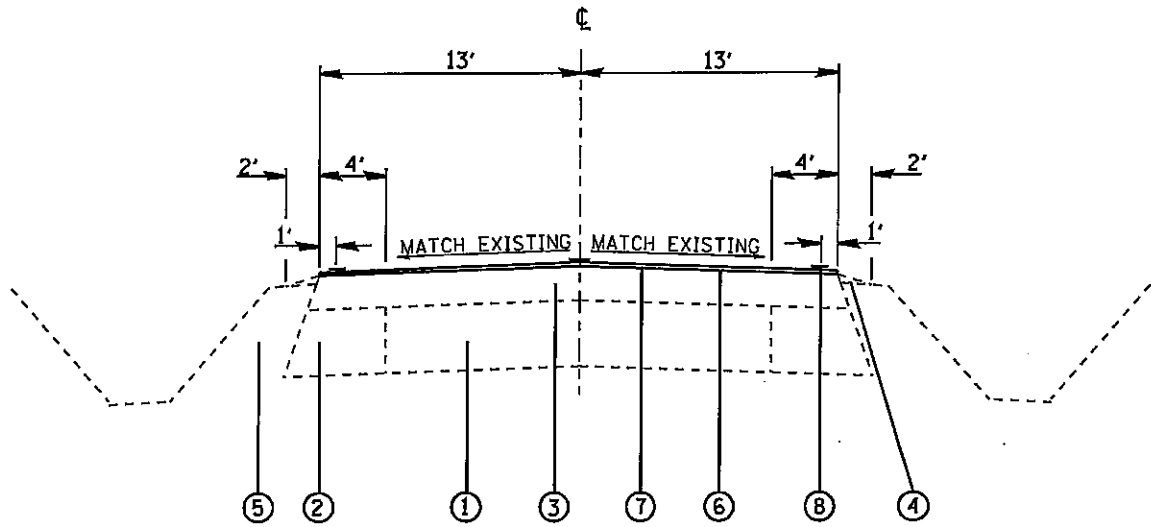
TYPICAL SECTION
