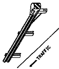
Standard Treatment - Direct Applied Sheeting Traffic Barrier Terminal Type 1 (Special)
