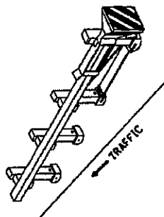
Standard Treatment - Direct Applied Sheeting Traffic Barrier Terminal Type 1 (Special)
