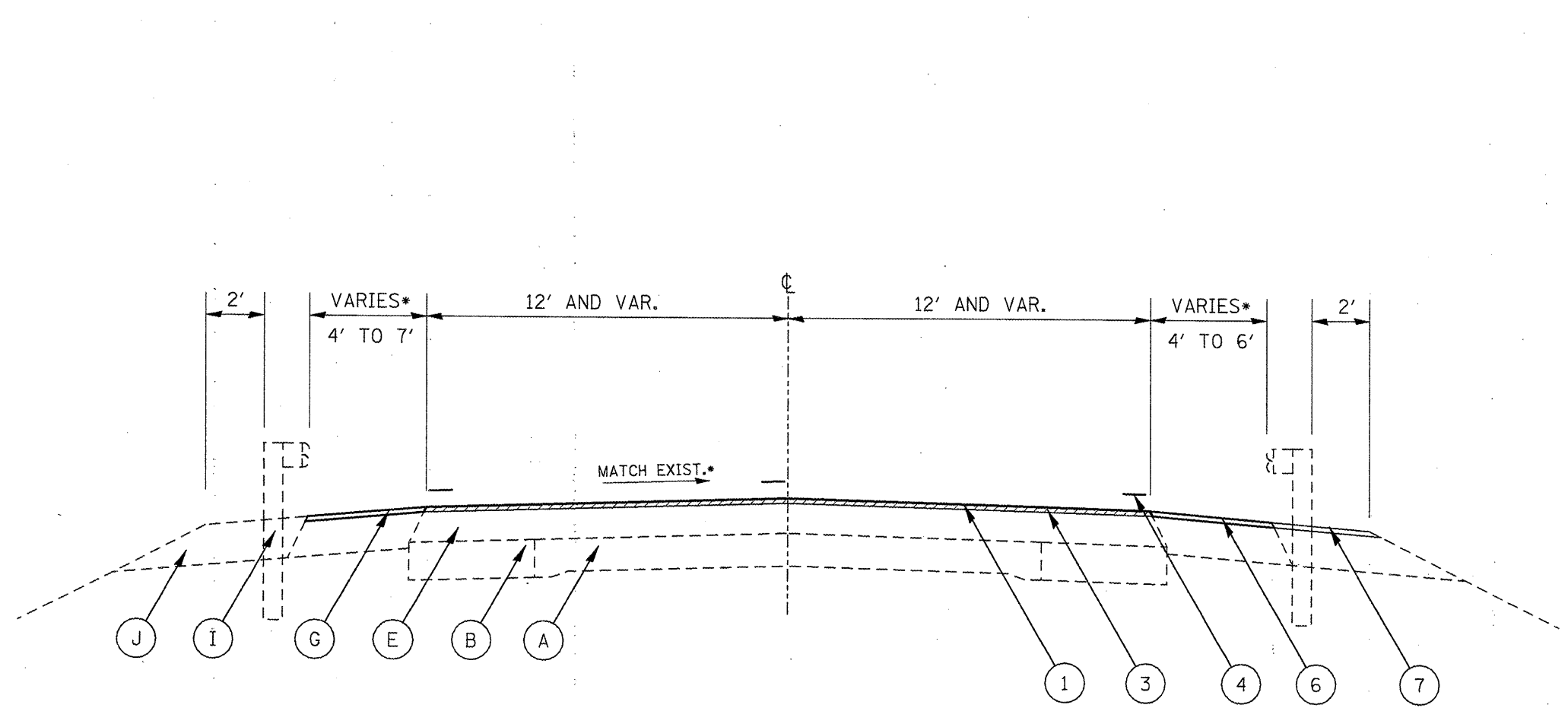
IL 89 TYPICAL SECTION 6 SEE NOTE SHEET 4
