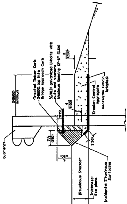
TYPICAL SECTION WITH EROSION CONTROL CURB
