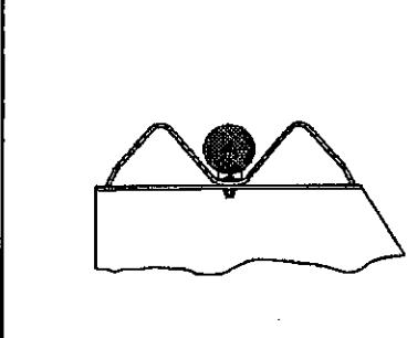
TYPICAL GUARDRAIL MOUNTING WITH REFLECTOR MARKER TYPE A
