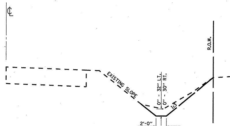
TYPICAL DITCH DETAIL
