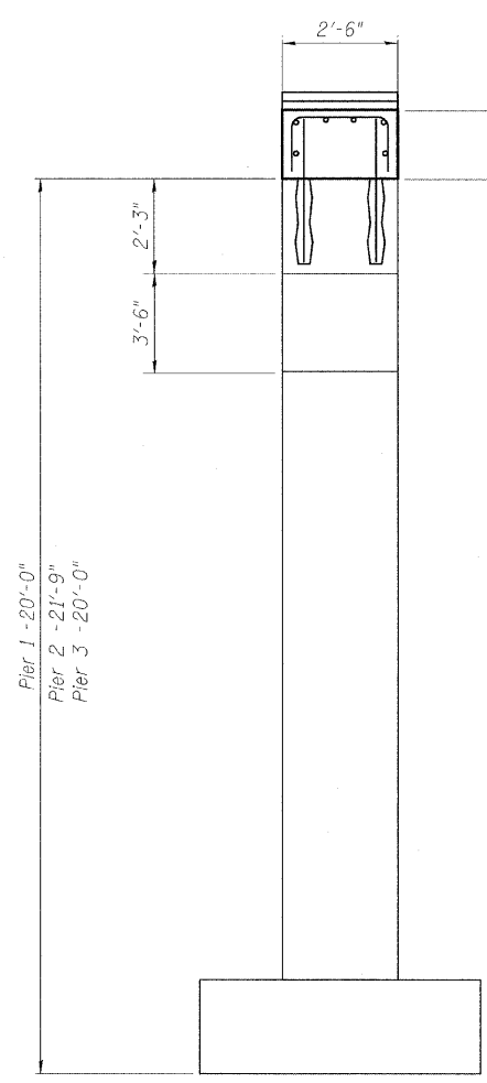
END VIEW
