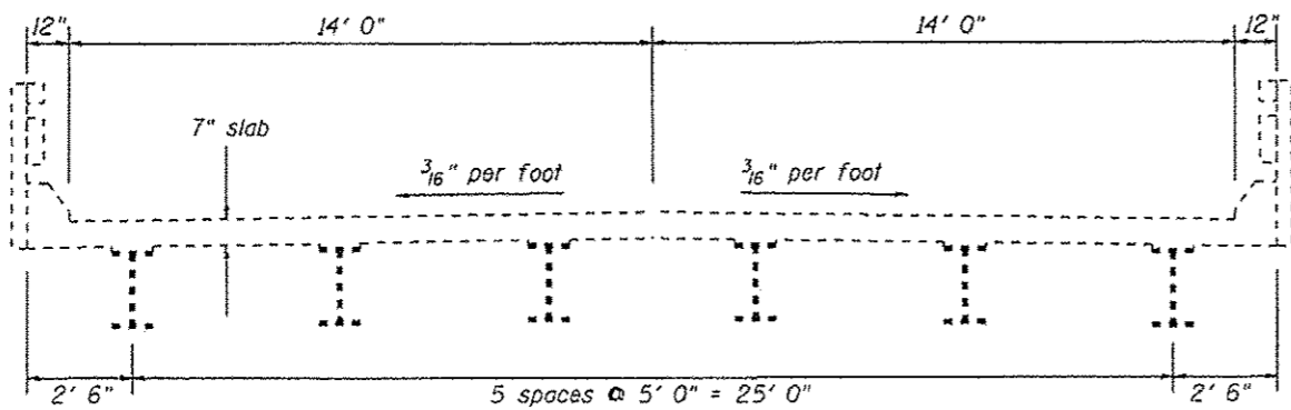
CROSS SECTION - SPANS 9-13
