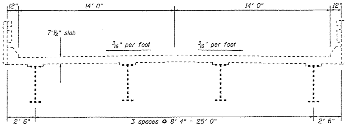
CROSS SECTION - SPANS 1-8 & 14-17
