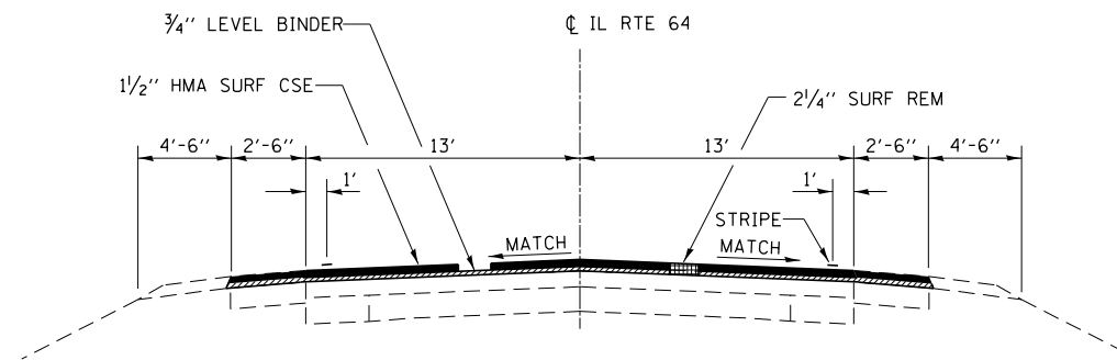
TYPICAL SECTION 8
