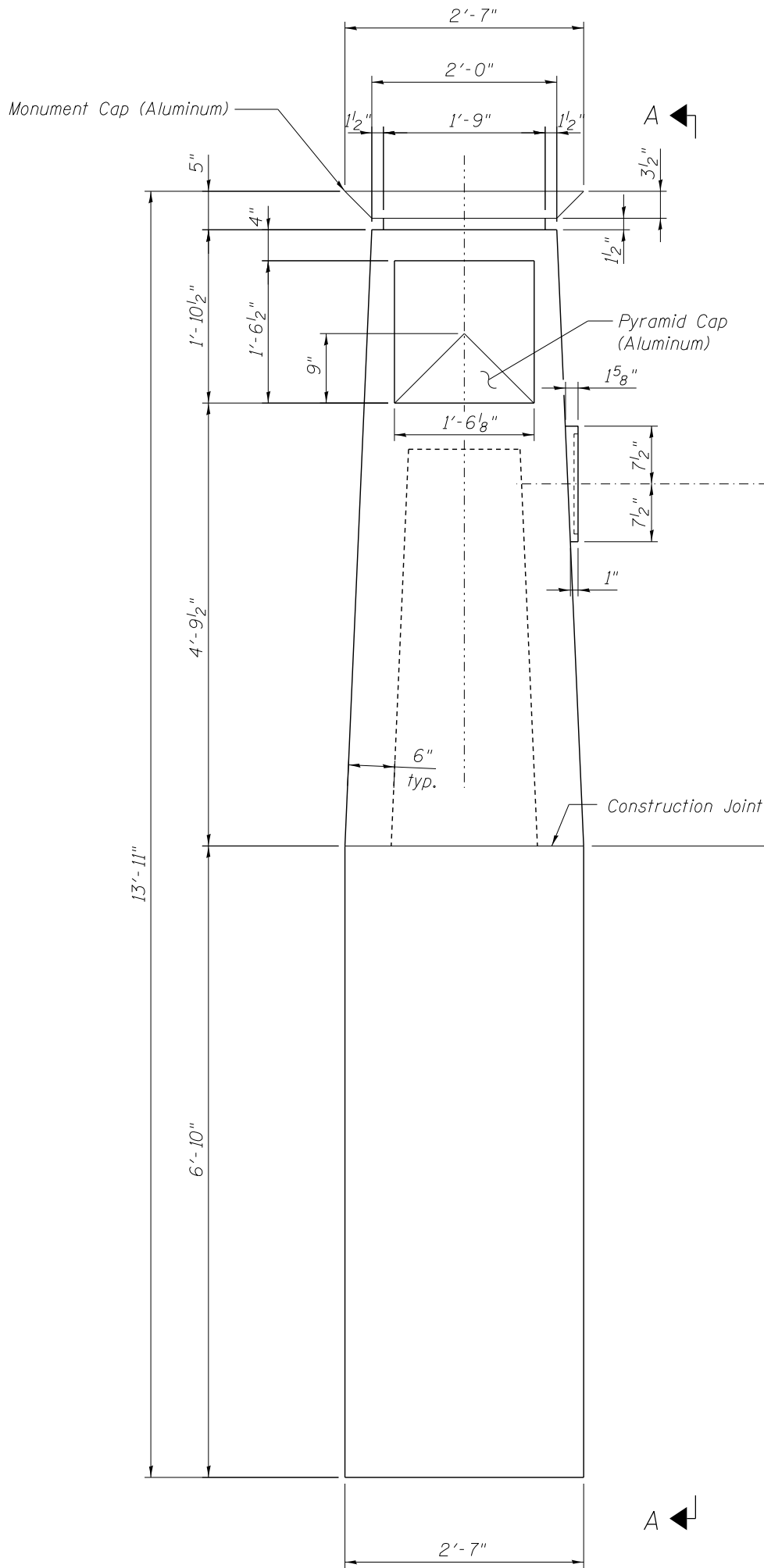
MONUMENT ELEVATION
