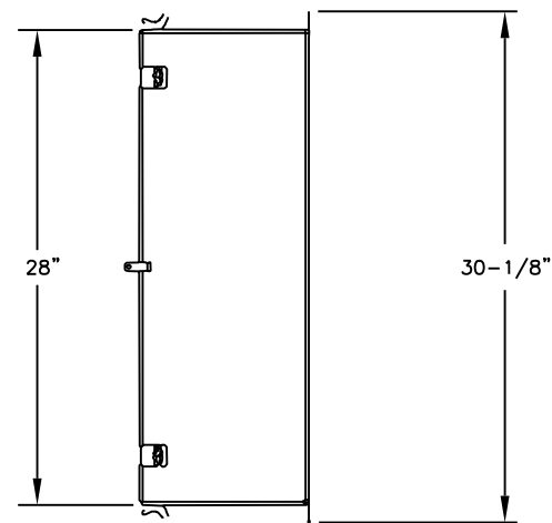
5 HUB - SIDE VIEW SCALE: NOT TO SCALE
