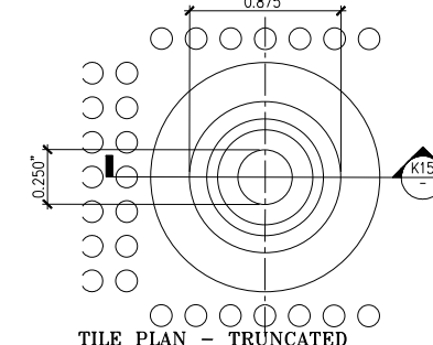
K11 TILE PLAN - TRUNCATED DOME FASTENER LOCATION SCALE : 1:1
