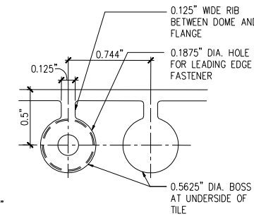
K8 PLAN AT U/S OF FASTENER SCALE : 2:1
