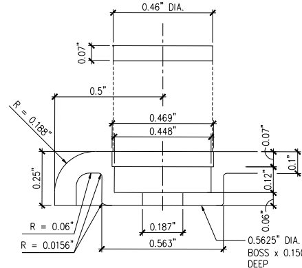
K5 CAP DETAIL SCALE : 4:1
