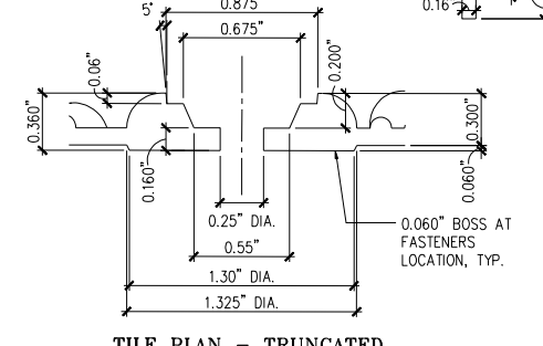
K15 TILE PLAN - TRUNCATED DOME FASTENER LOCATION SCALE : 1:1
