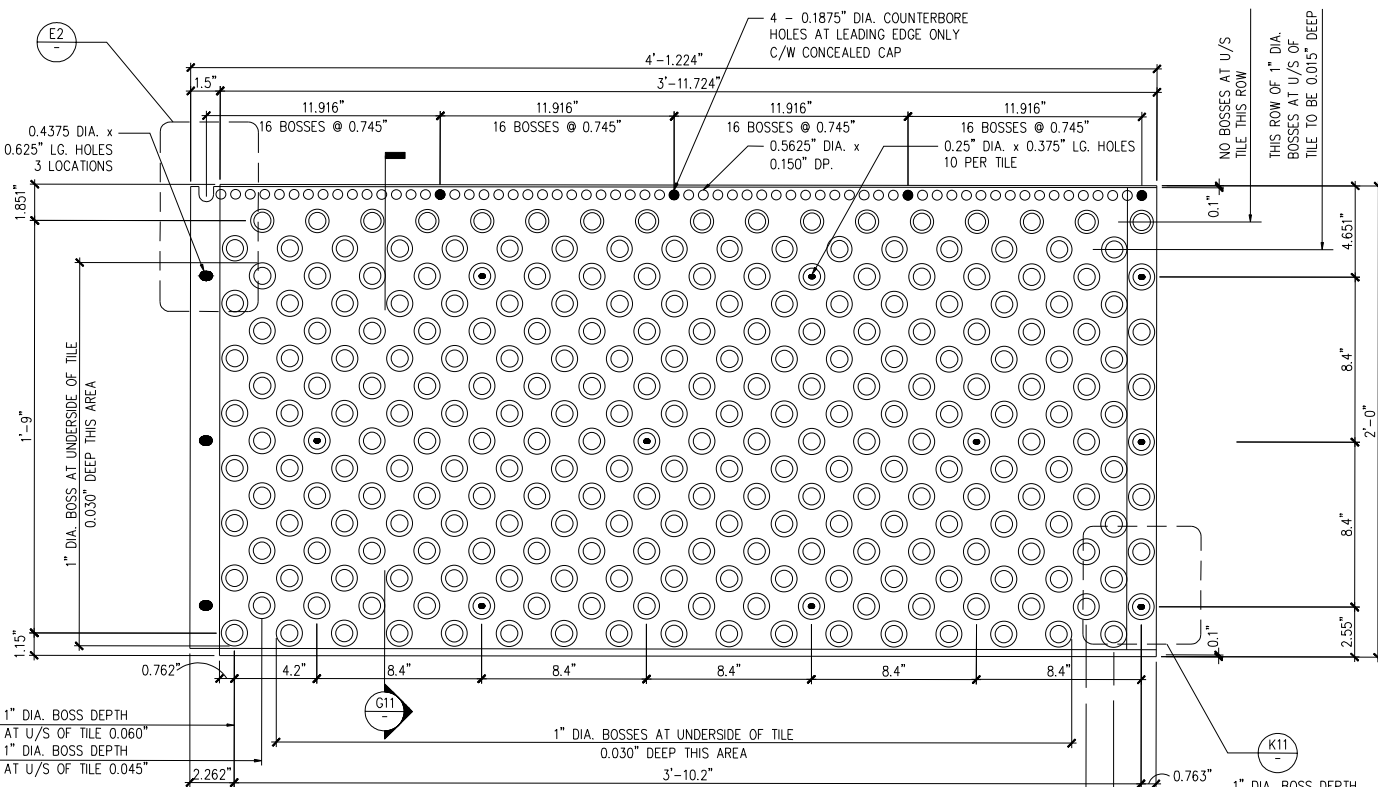
E11 PLAN - TILE SCALE : 3" = 1'-0"
