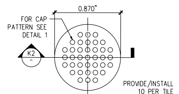
J2 PLAN - T/O CONCEALED CAP SCALE : 2:1
