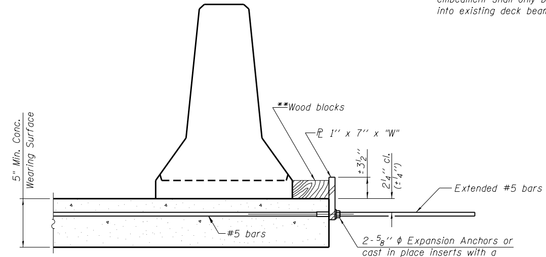
DETAIL II
