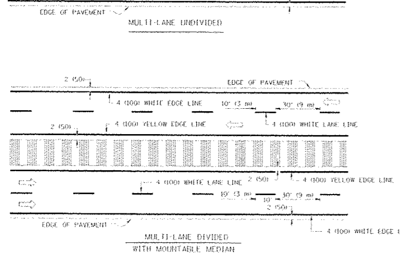
TYPICAL LANE AND EDGE LINE MARKING
