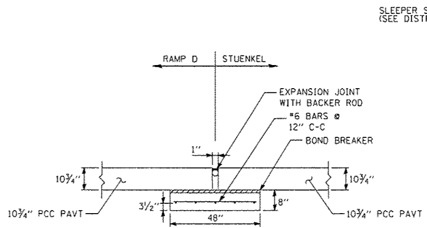
1 INCH EXPANSION JOINT WITH SLEEPER SLAB
