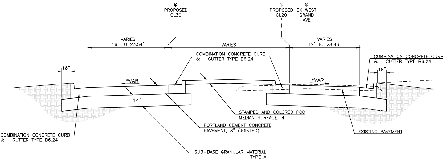
TO BE USED STA 21+44.42 TO STA 23+31.16 (CL20)
