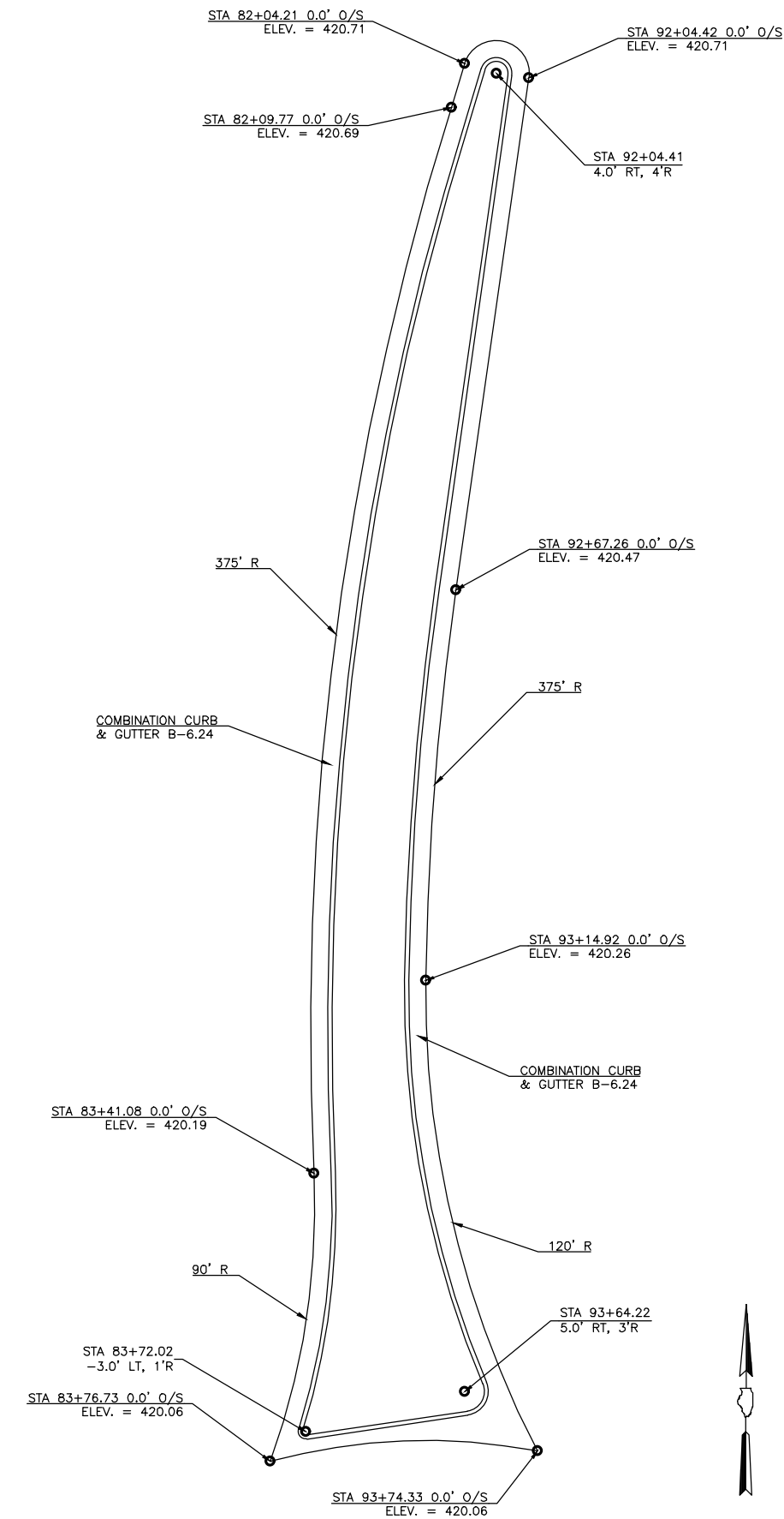
NORTH SPLITTER ISLAND
