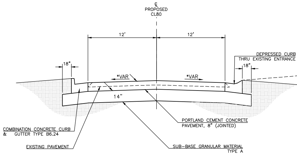
TO BE USED STA 80+00 TO 81+00 (CL80)
