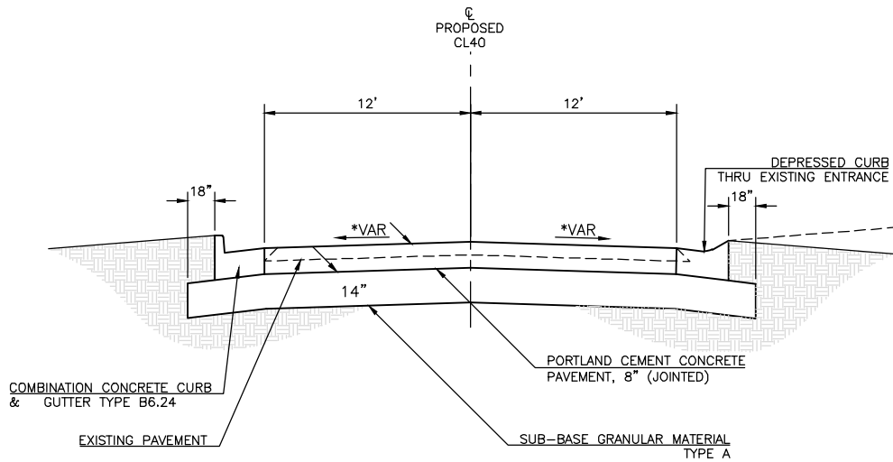
TO BE USED STA 50+00 TO 51+73.70 (CL50)
