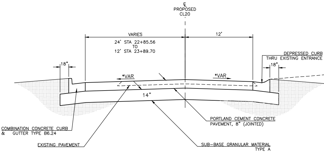
TO BE USED STA 23+89.70 TO 23+59.62 (WEST GRAND AVE)
