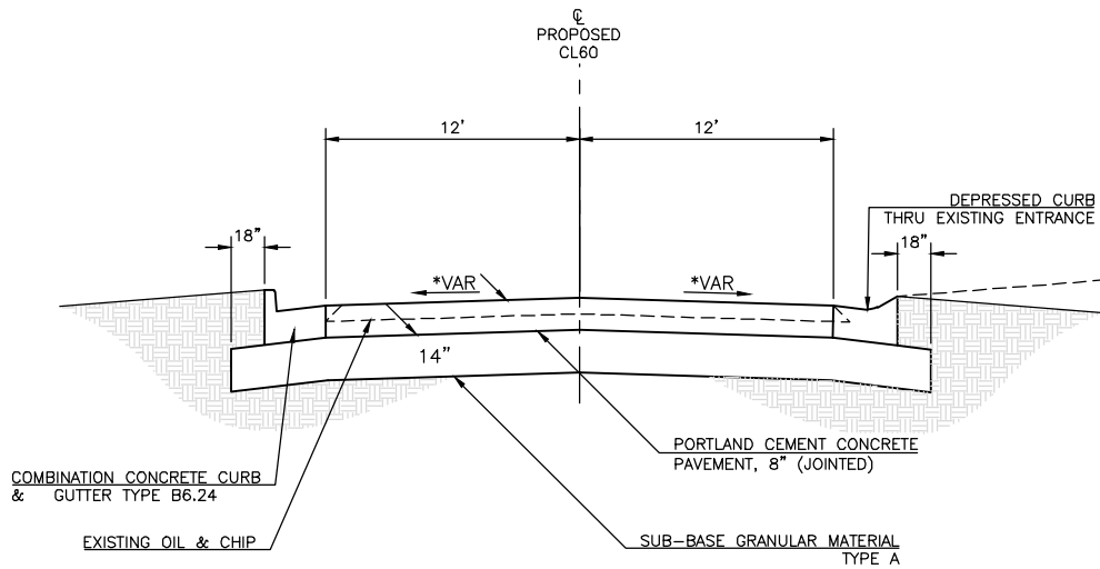
TO BE USED STA 60+00 TO 61+17.07 (CL60)
