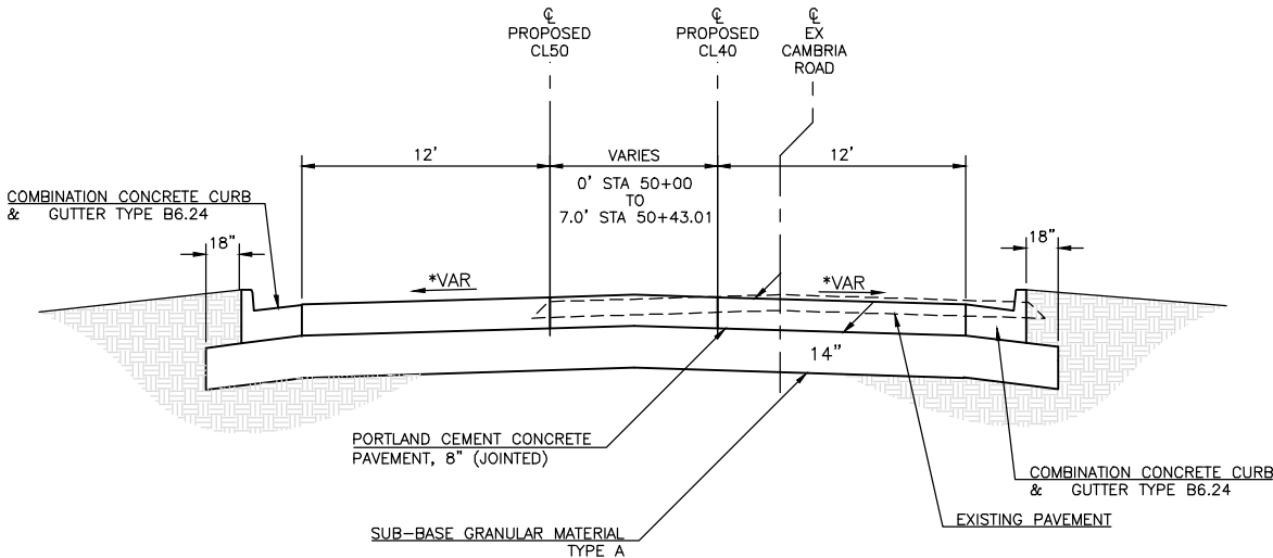
TO BE USED STA 50+73.70 TO STA 51+43.01 (CL50)
