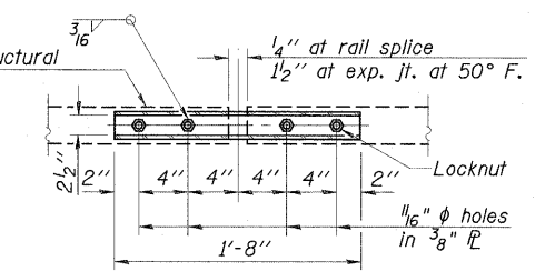
PLAN-BOTT. SPLICE PL TYPICAL
