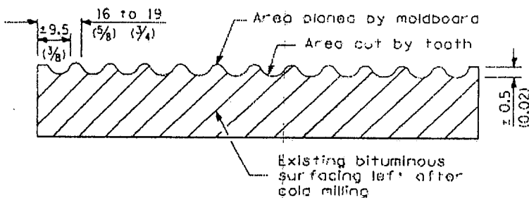
SECTION B-B PROJECTED PERPENDICULAR TO CENTERLINE
