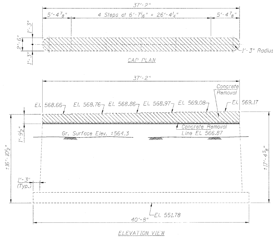
CONCRETE REMOVAL DETAILS - EXISTING PIER 2 - W.B.L. (W.B.L. - Looking East - UpStation)
