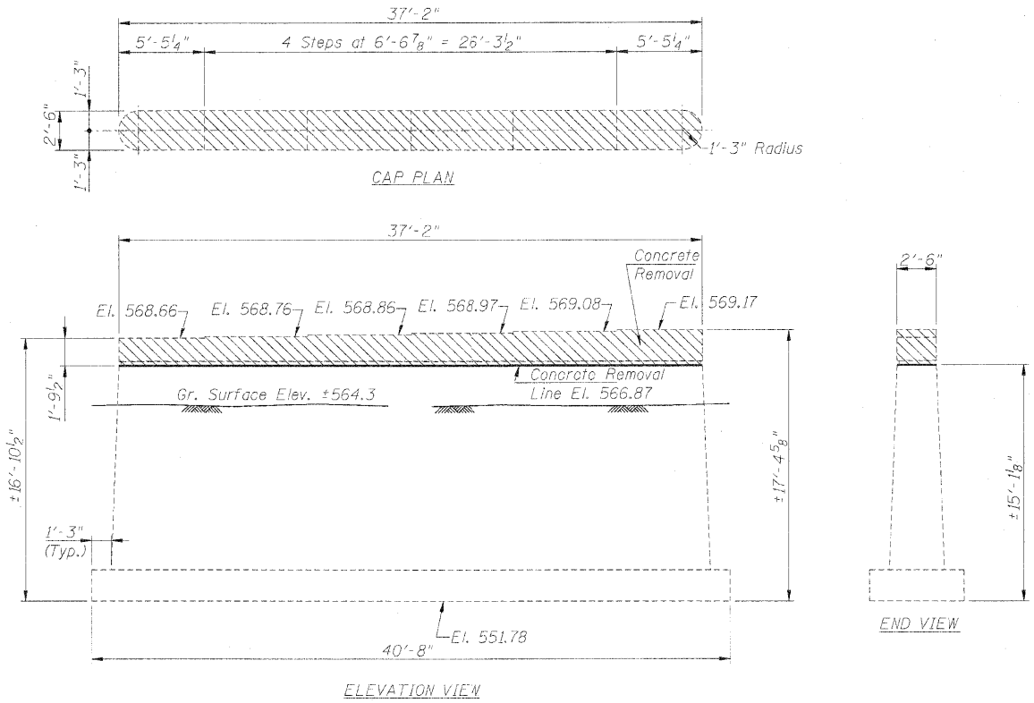
CONCRETE REMOVAL DETAILS - EXISTING PIER 5 - E.B.L. (E.B.L. - Looking East - UpStation)
