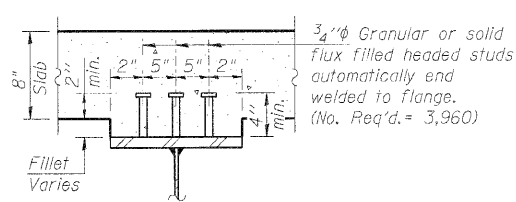
6" Abutment Brgs. 4" 4" x 2" x 2" SloTTed Holes Web 4"
