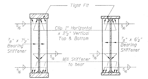
BRG. STIFFENERS AT ABUTMENTS
