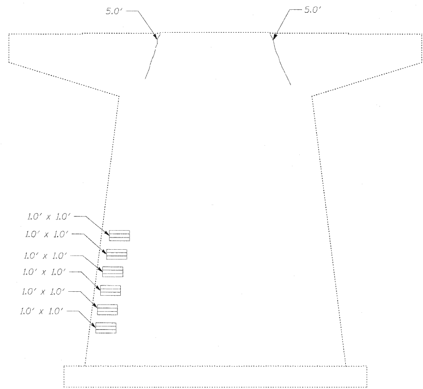
EAST ELEVATION (Looking West)
