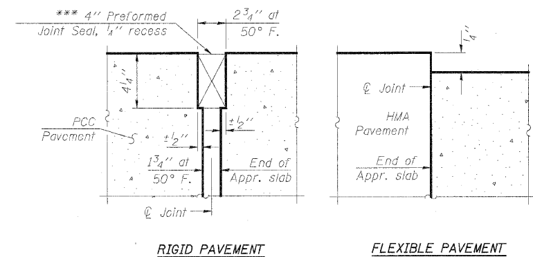
DETAIL C
