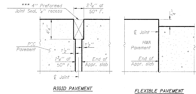
DETAIL C
