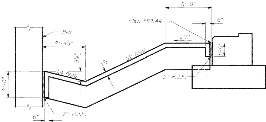
SECTION THRU EAST SLOPEWALL (Looking North)
